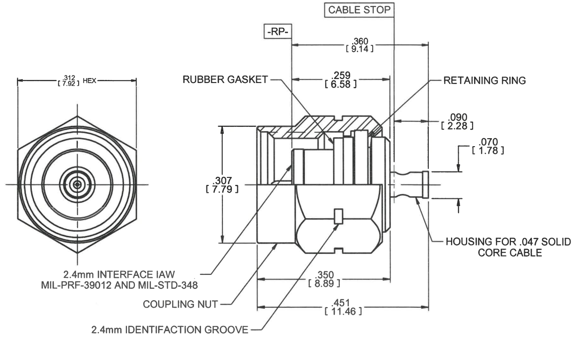
CABLE TERMINATION END
