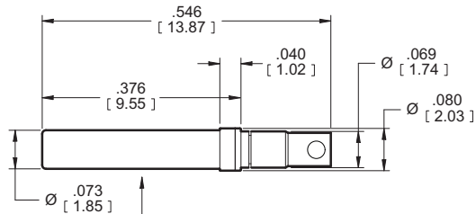
SSBP Size 20HD Socket Assembly (Female)
