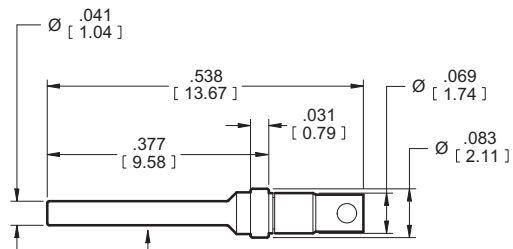
SSBP Size 20HD Pin Assembly (Male)
