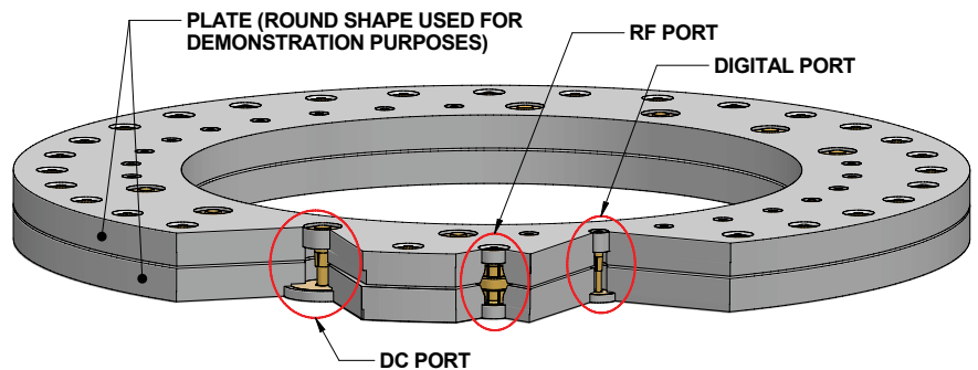
Cross-section view of custom design. Southwest Microwave SSBB RF connectors can be built onto any plate shape with DC and digital ports.
