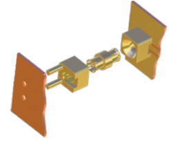
Board-to-Board Application
