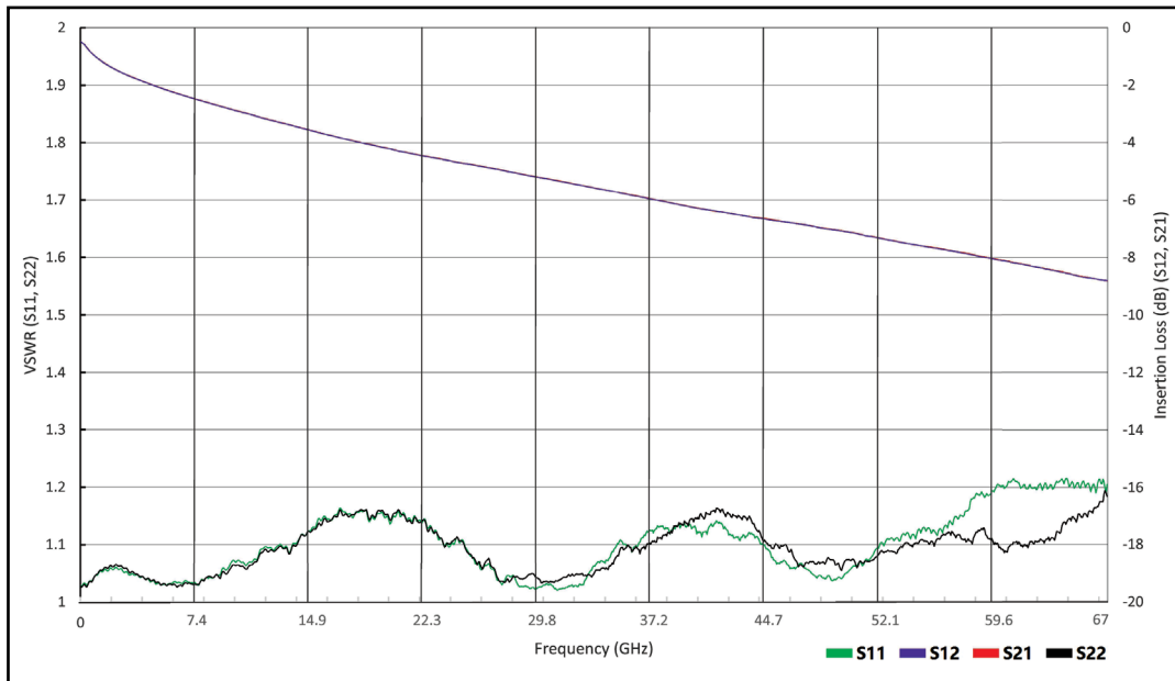
Typical Test Data - 1.85 mm Plug to SSBB J, 12 Inch Long Cable
