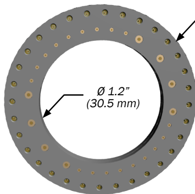
High Density Application (aerial view of custom design)
